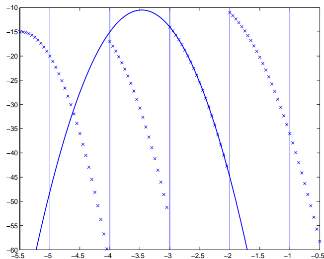
Figure 2-9: A Piecewise-Polynomial Function, Its Breaks, and the Polynomial Giving Its Third Piece
